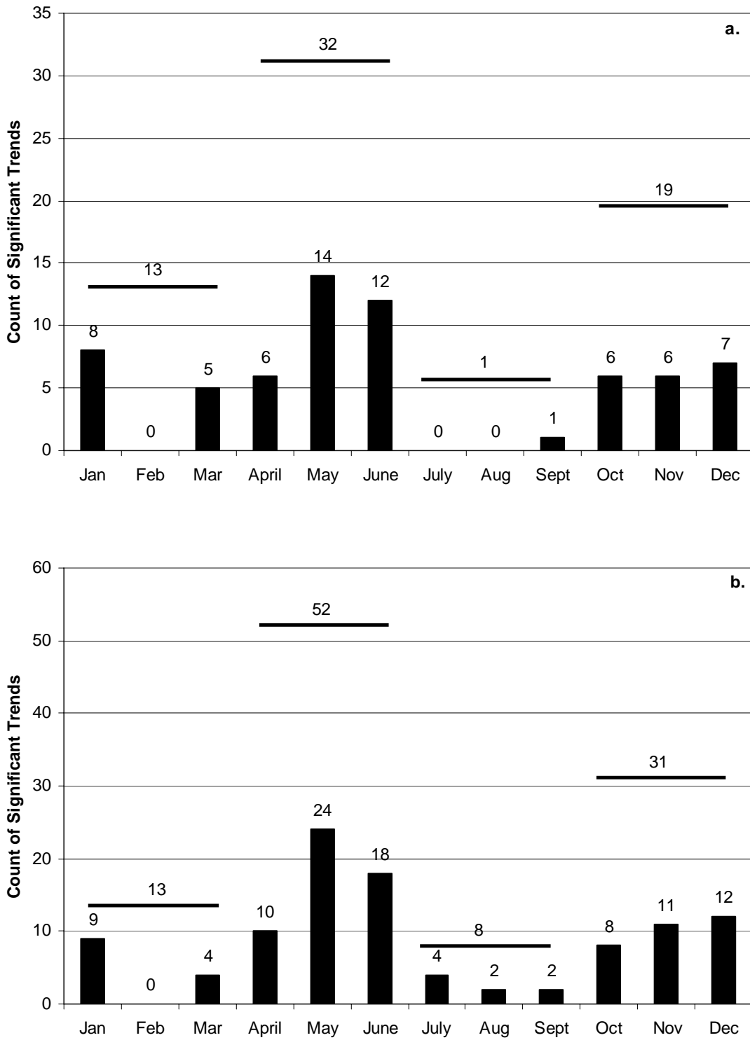
Figure 3.1 Distribution of months with positive trends that are significant at the (a) 95%, and (b) 90% level for MMRI. Lines indicate seasonal groupings for winter, spring, summer and fall.
