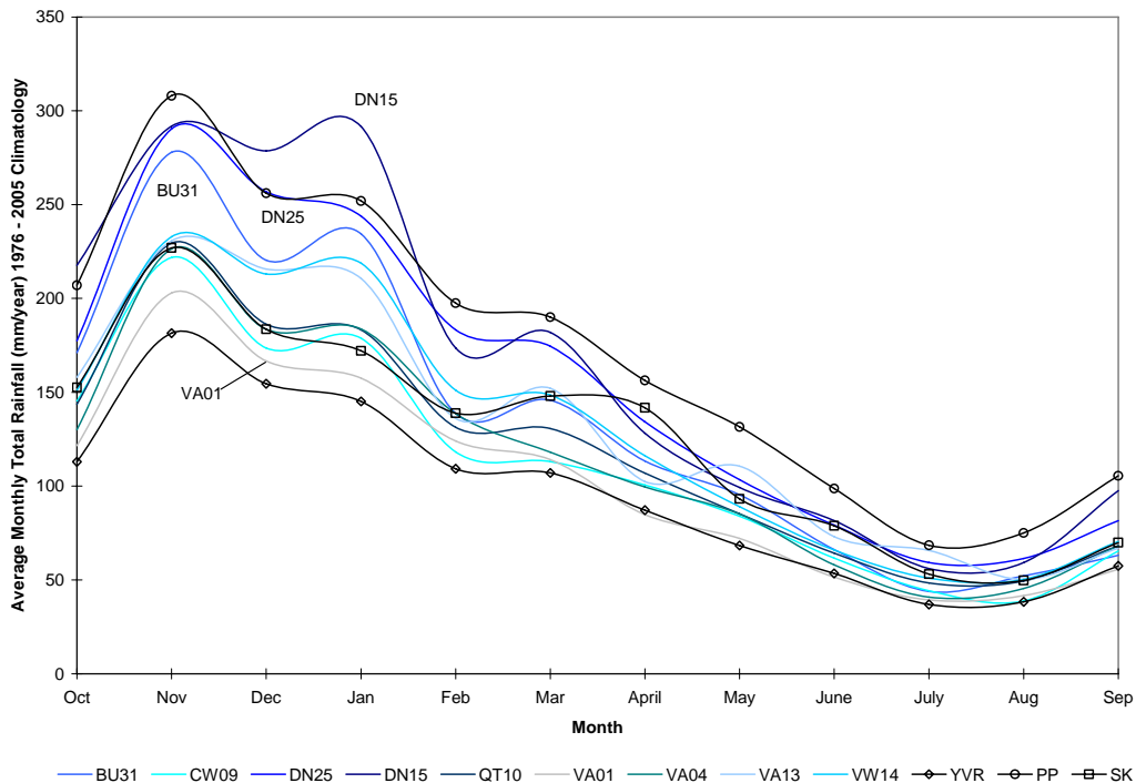
Figure 1.2 Monthly total rainfall, October to September for the GVRD stations and MSC stations, 1976–2005.
