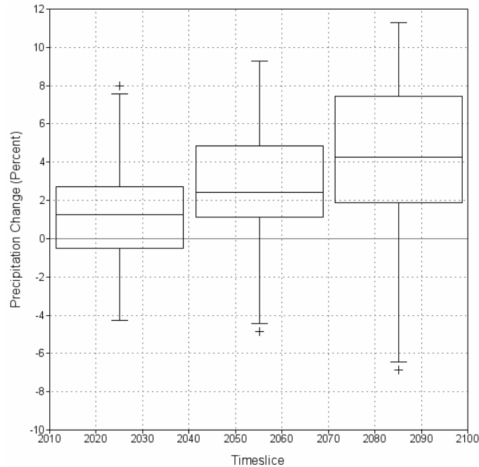
Figure 3.5 Box and whisker plot for the annual future precipitation projections for 2020s, 2050s and 2080s. See text for full explanation.
