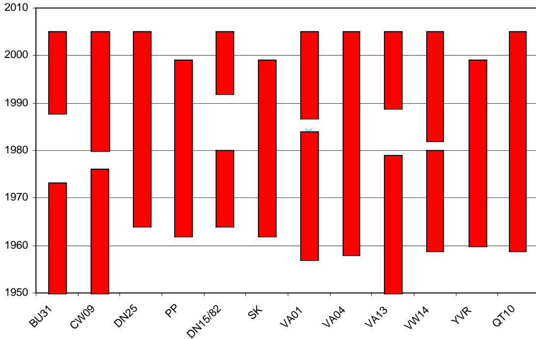
Figure 2.1 Plots of time periods used in the annual time series analysis. Gaps indicate missing or unavailable data.
