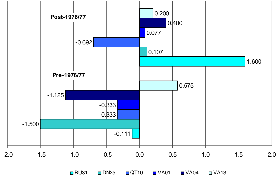
Figure 3.3 ATEC trends (occurrences per year) for the 5-minute duration, pre-76/77 and post-76/77.
