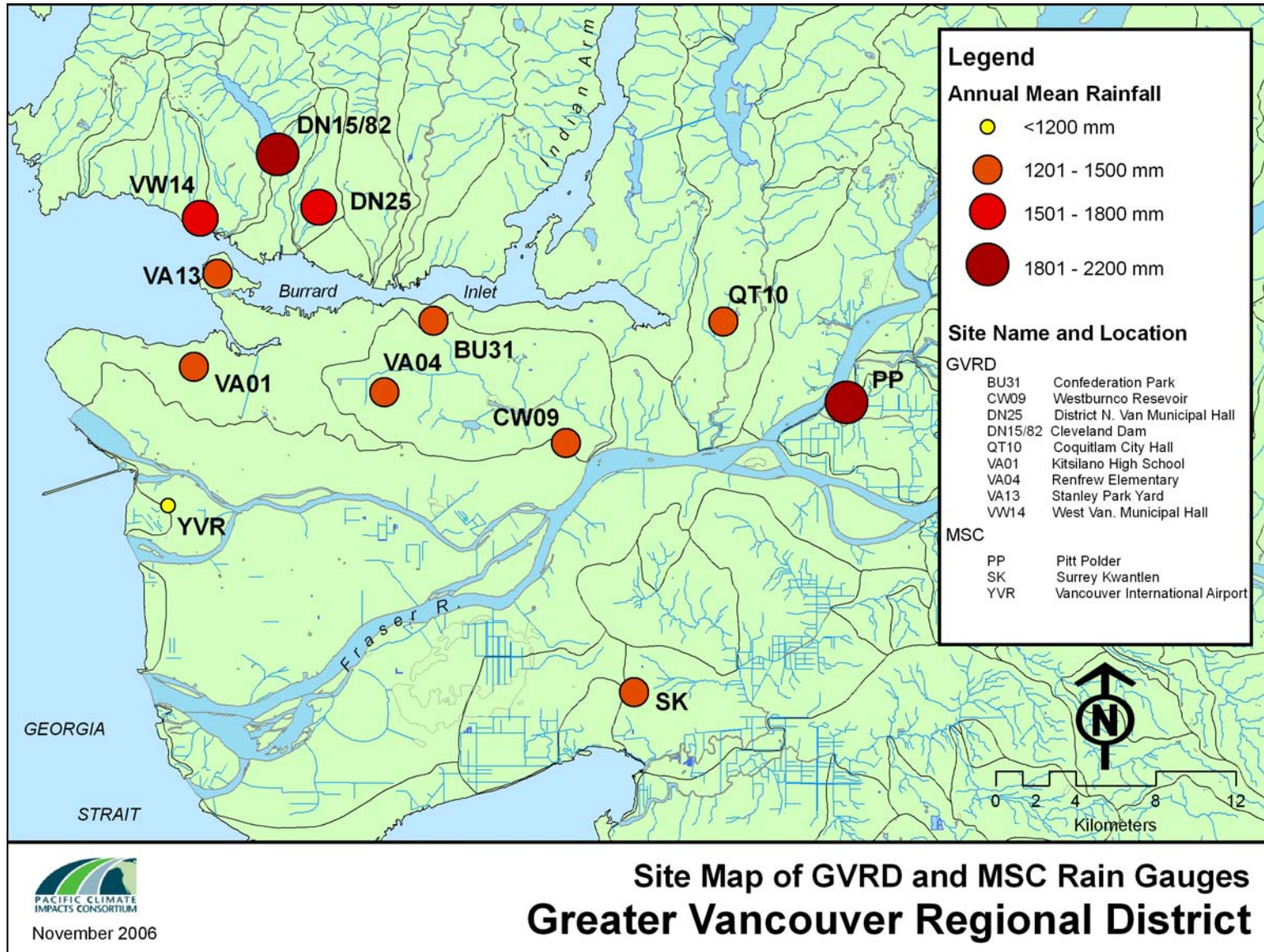
Figure 1.1 Map of rainfall station locations in the GVRD and annual mean rainfall amounts.
